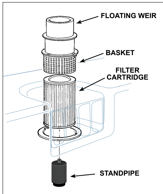
FILTER SYSTEM
